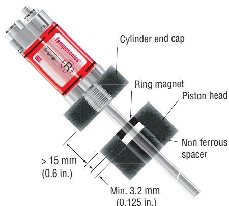
Figure 10. Model RH rod-style mounting
