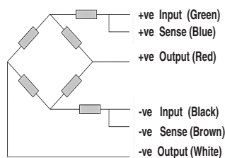
Wiring Schematic Diagram (Balanced temperature compensation)
